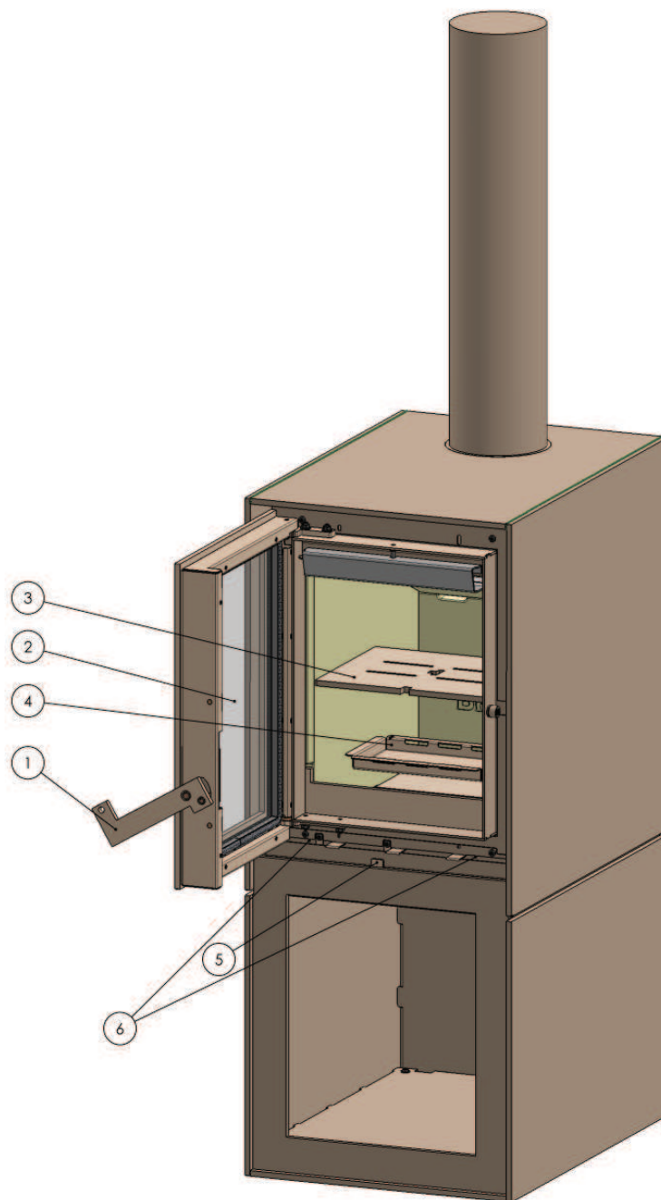
Figure 2: Operation Box with log store
