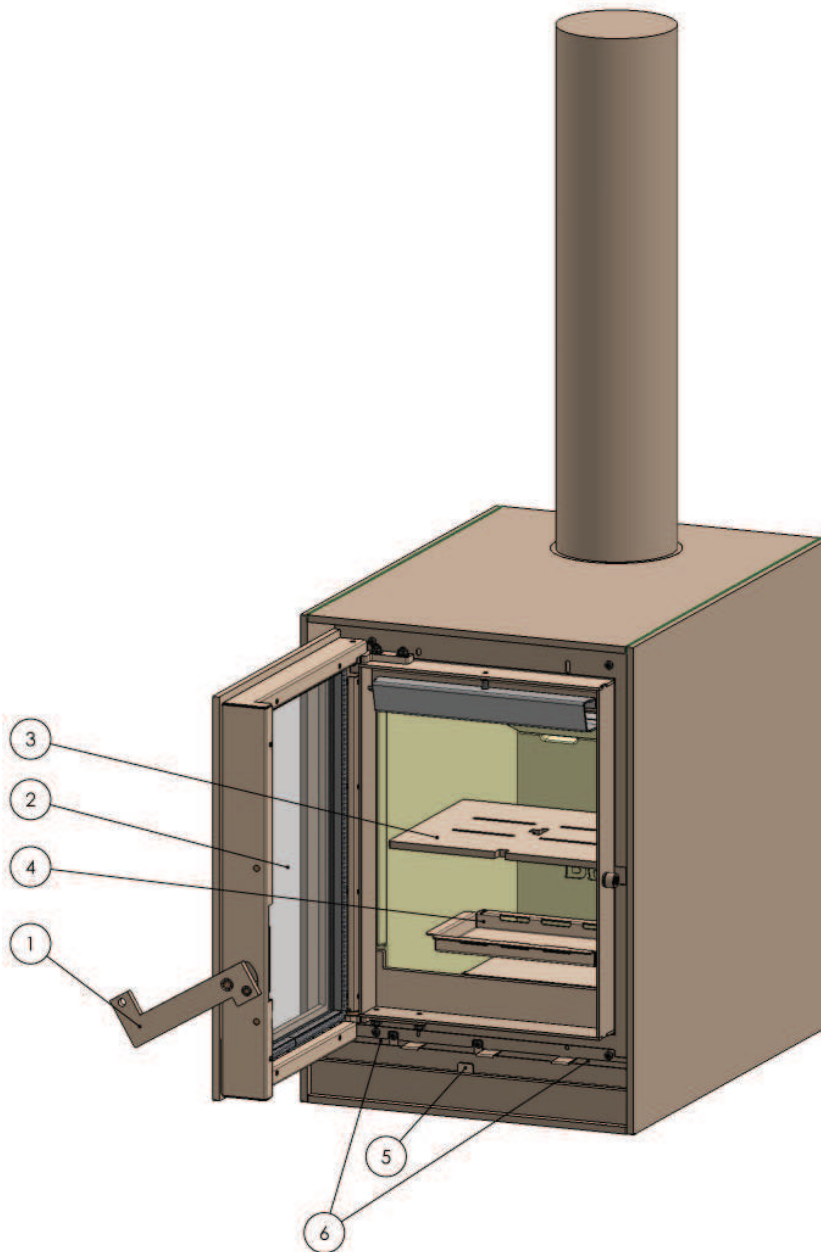
Figure 1: Operation Box
