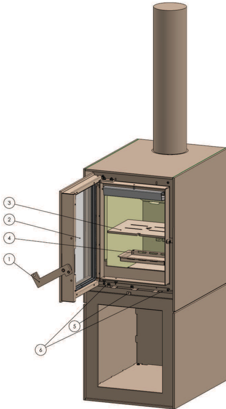
Figure 2: Operation Box with wood log store module
