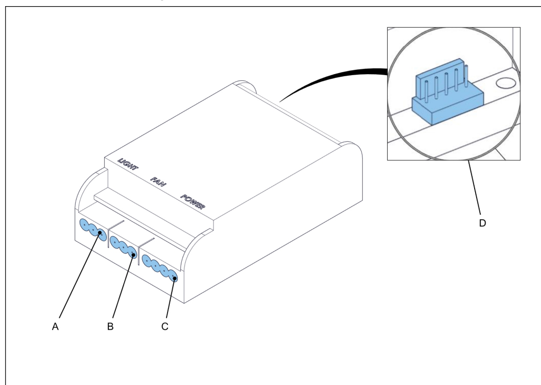
Figure 1. Fan/light module
