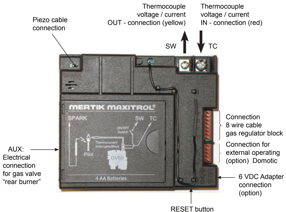
Figure 25: Receiver - Top
