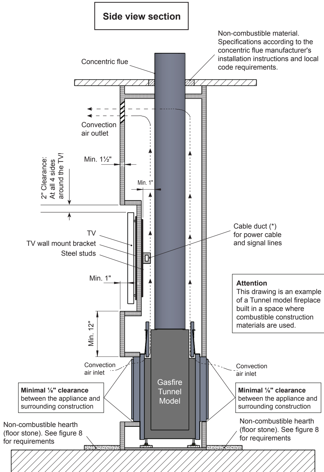
Figure 12: TV installation directly above offset tunnel fireplace (Recessed mounted) Side View Section
