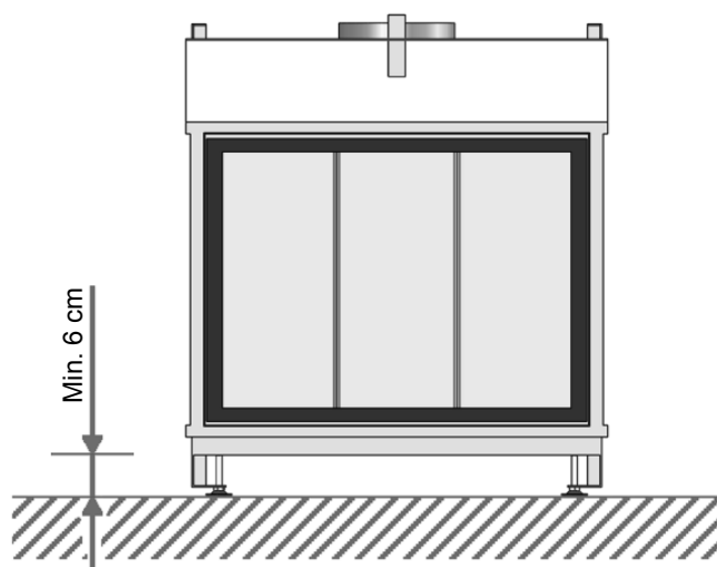
Figure 15: A clearance of at least 6 cm must be maintained between the bottom plate of the appliance and the floor.
