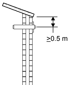
Figure 2: Wall-mounted outlet
