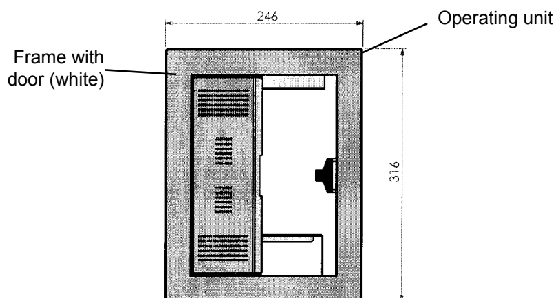
Figure 18: Operating unit
