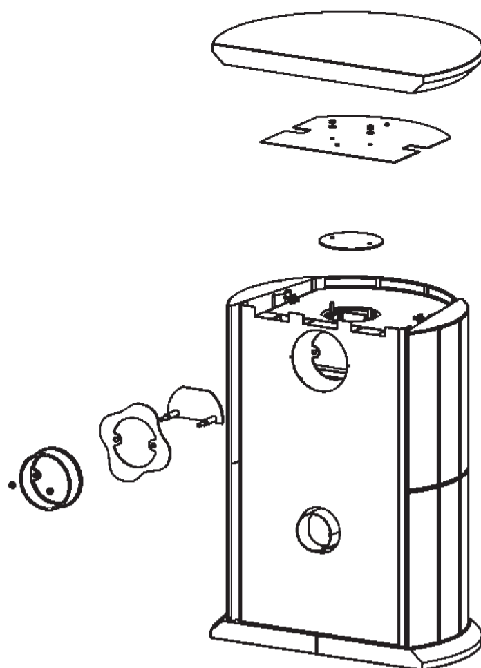
Figure 2: Rear connection
