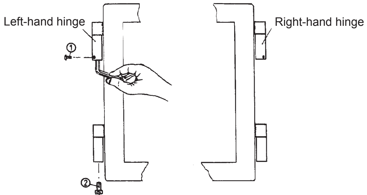
Figure 4: Hinges
