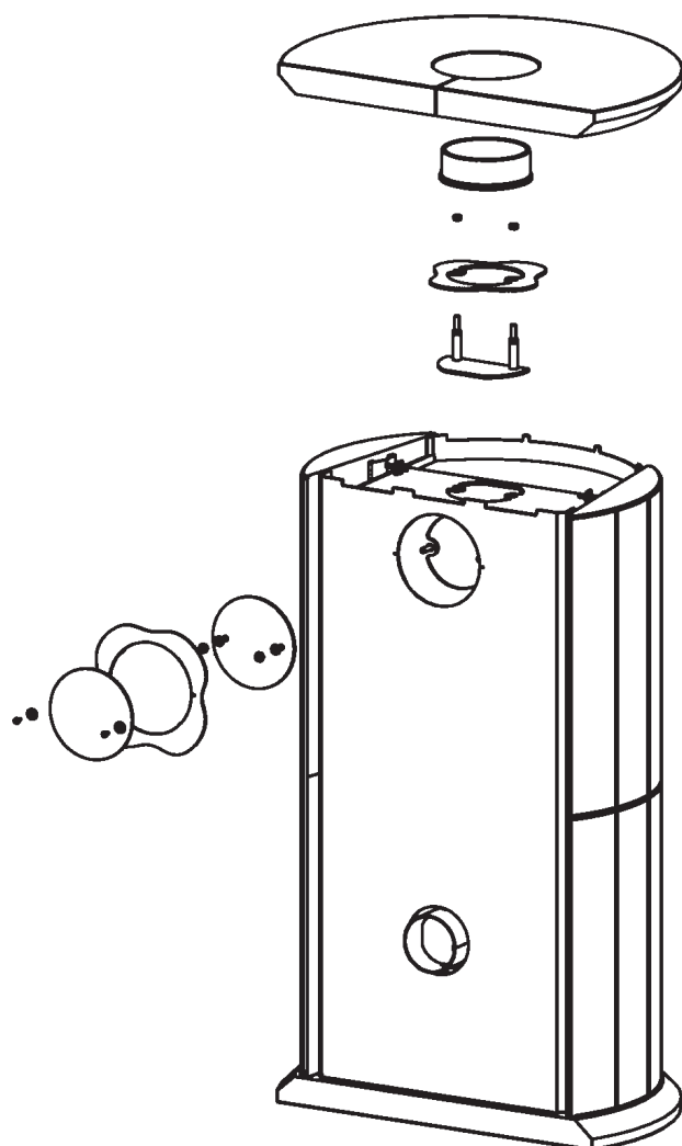
Figure 1: Raccord supérieur
