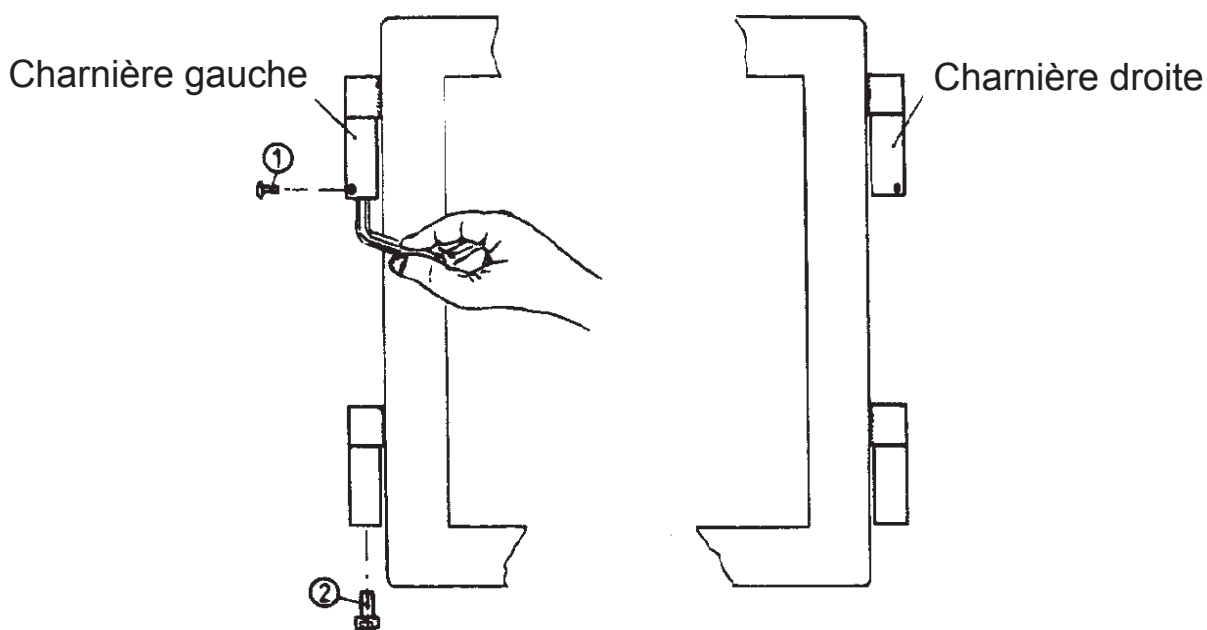
Figure 4: Charnières
