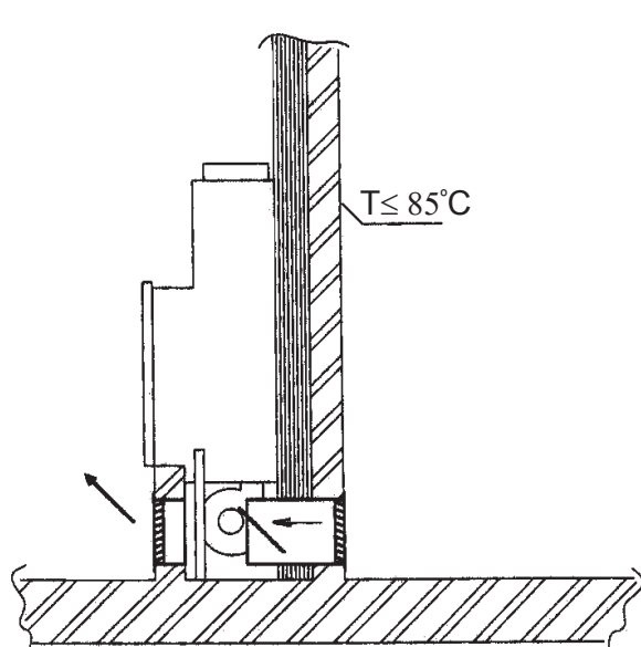
Fire against a non-bearing and non-flammable wall
