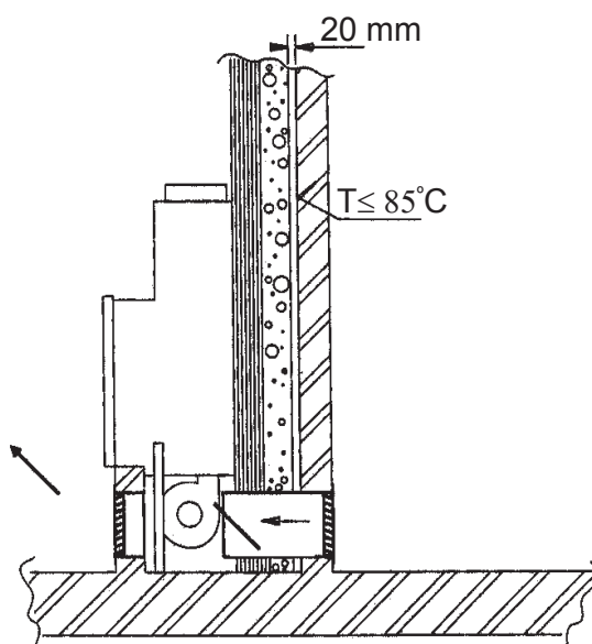
Fire against a bearing wall or wall with flammable material
