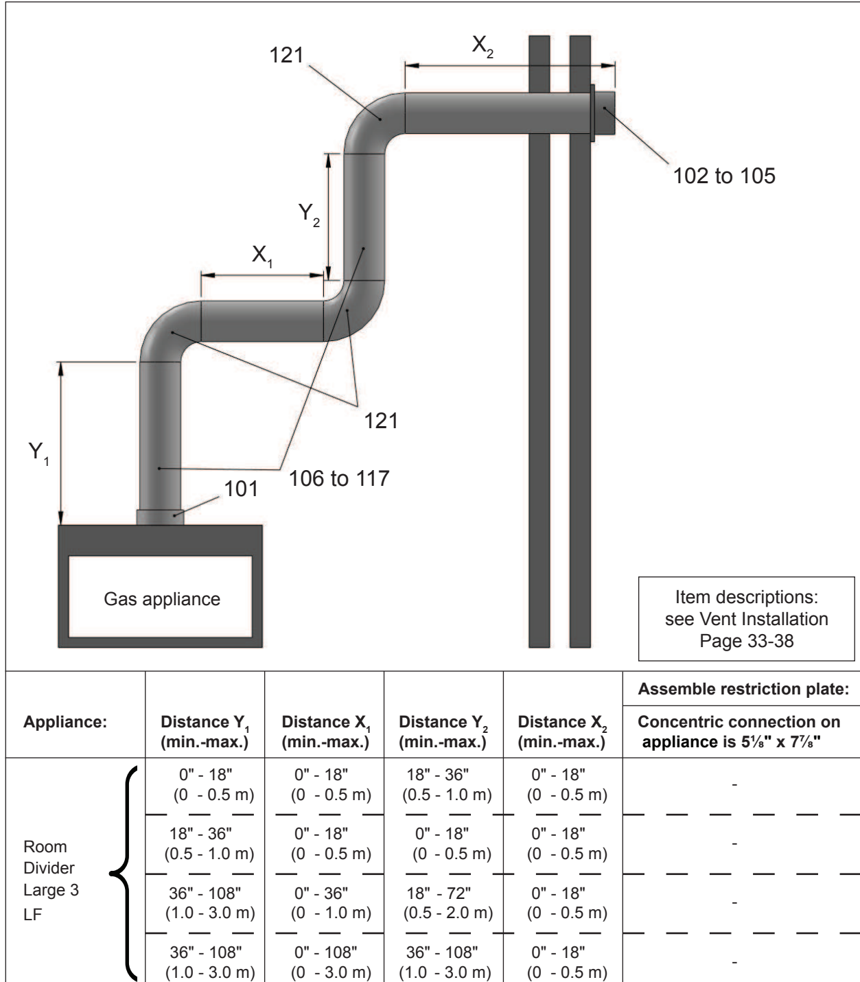
Figure 19: Horizontal wall termination
