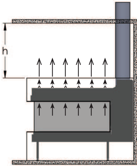
Floor standing / built-in: Example 3
