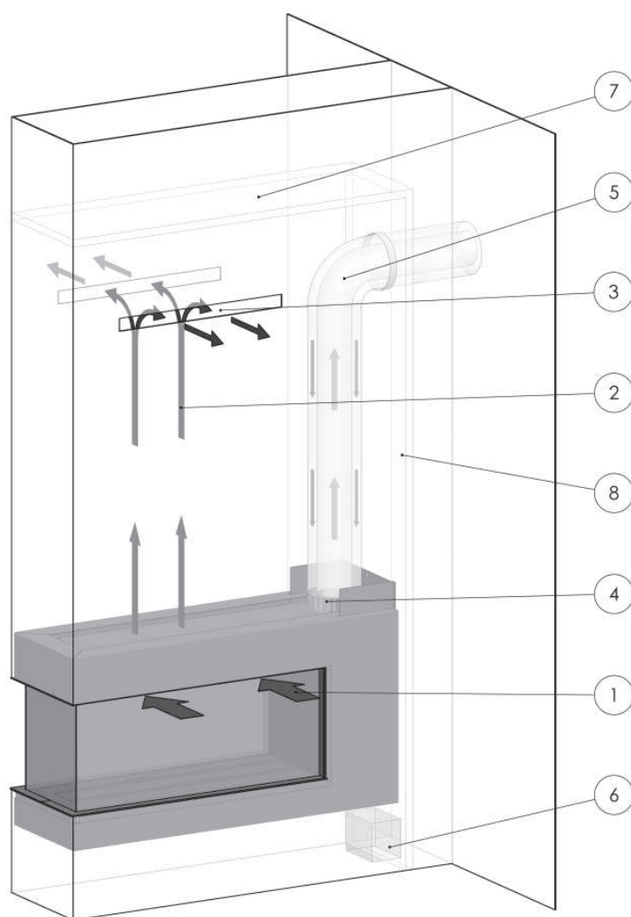
Figure 21: Appliance installed in ventilated chimney breast / Enclosure Horizontal outlet of the flue gas exhaust / combustion air supply via the wall.
