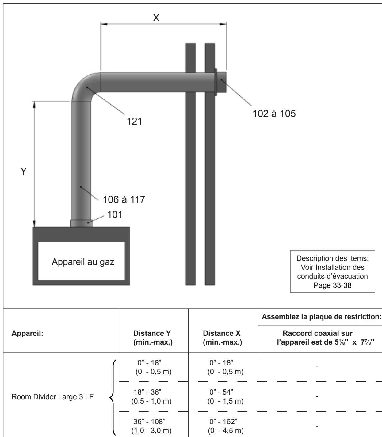
Figure 20: Terminaison murale horizontale
