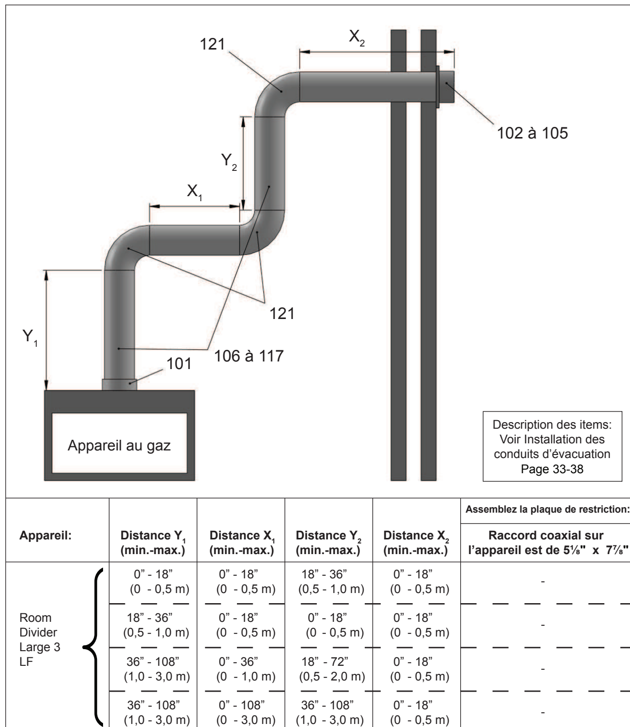
Figure 19: Terminaison murale horizontale
