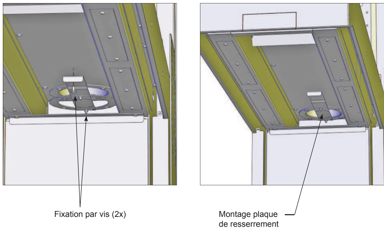
Figure 30: Place de la plaque de resserrement
