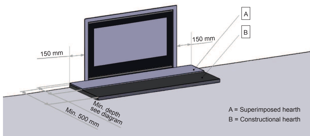
Figure 1: Minimum dimensions appliance
