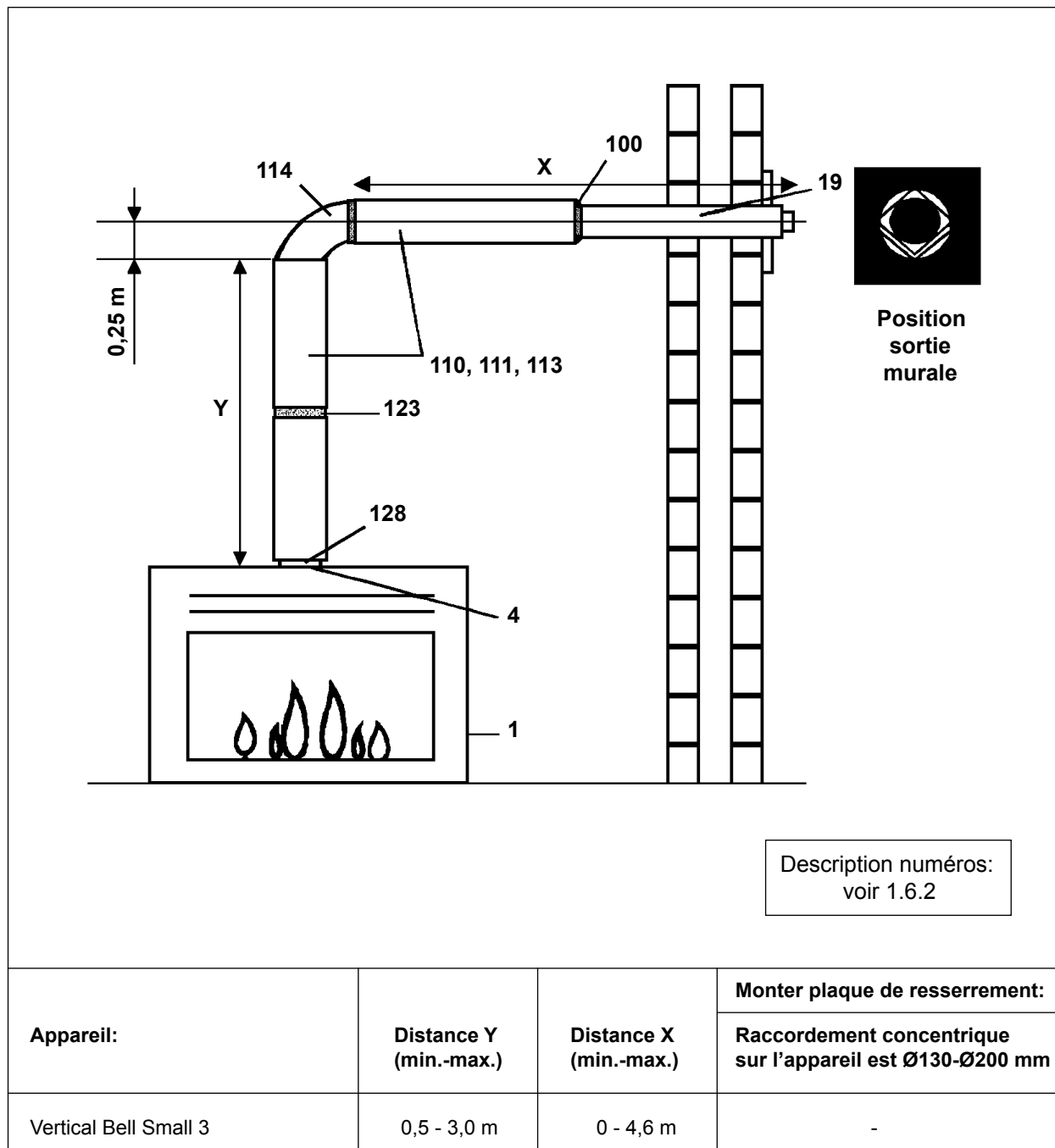
Figure 12: Sortie murale horizontale
