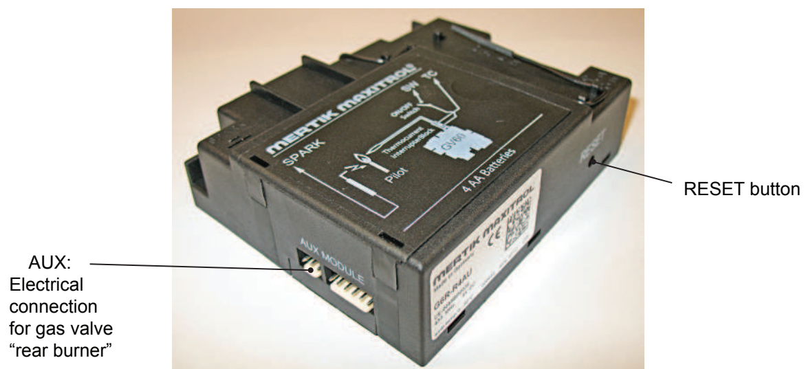
Figure 26: Receiver - AUX connection - RESET button
