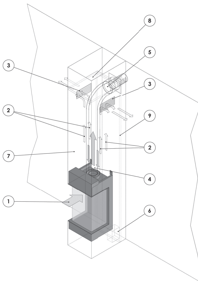
Figure 15: BUILT-IN APPLIANCE: Appliance installed in ventilated chimney breast / Enclosure Horizontal outlet of the flue gas exhaust /combustion air supply via the wall • Fitted with the accessory: high adjustable feet
