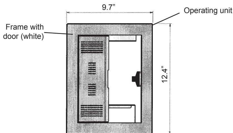
Figure 20: Operating unit
