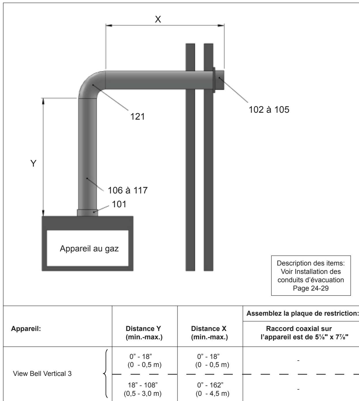
Figure 14: Terminaison murale horizontale
