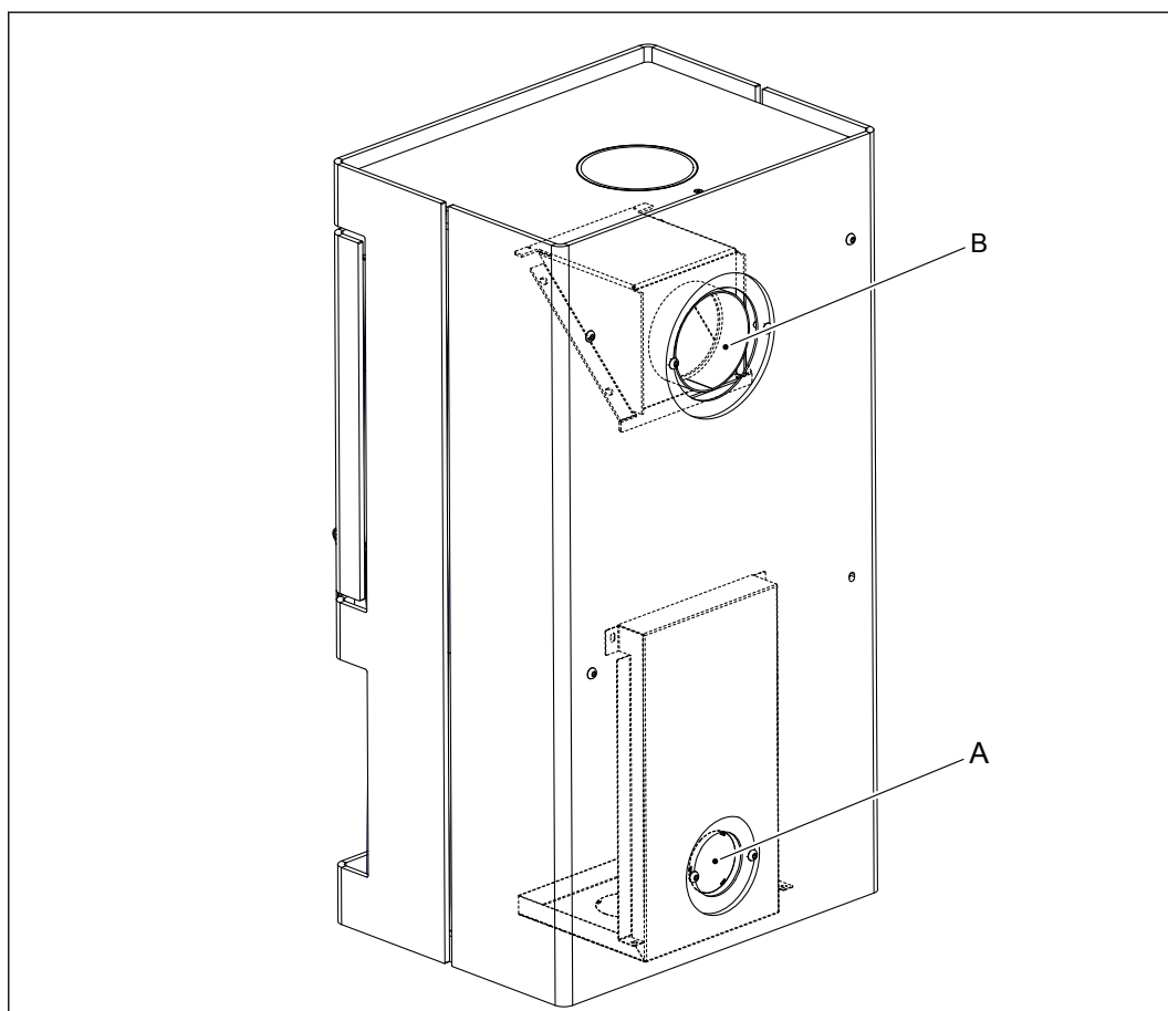
A Connection for external combustion air supply B Rear flue connection
