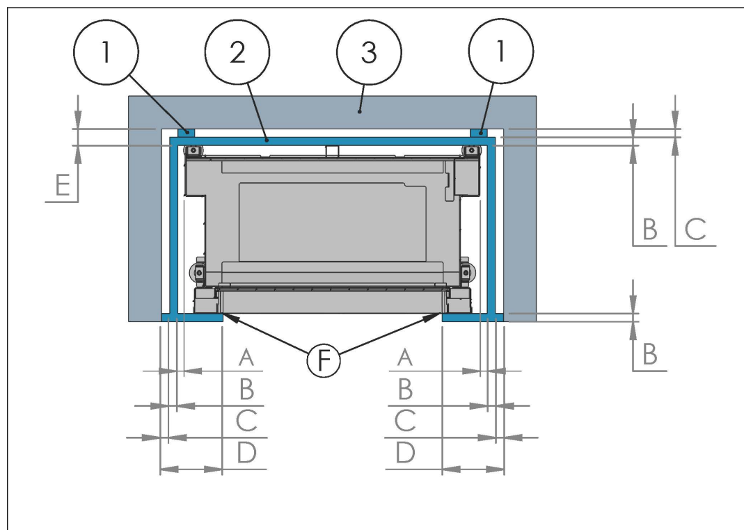
1 Non-flammable spacer 3 Flammable wall 2 Non-flammable insulation plate
