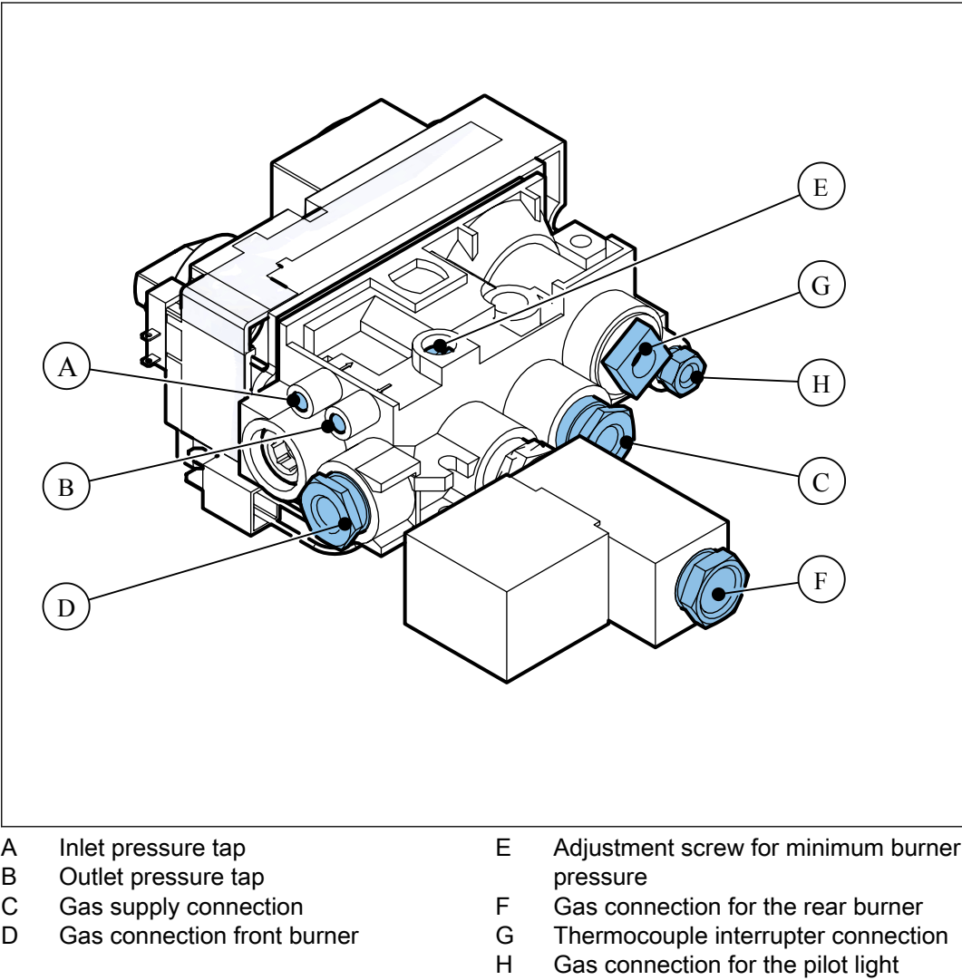
Figure 5. Gas regulator block (rear)
