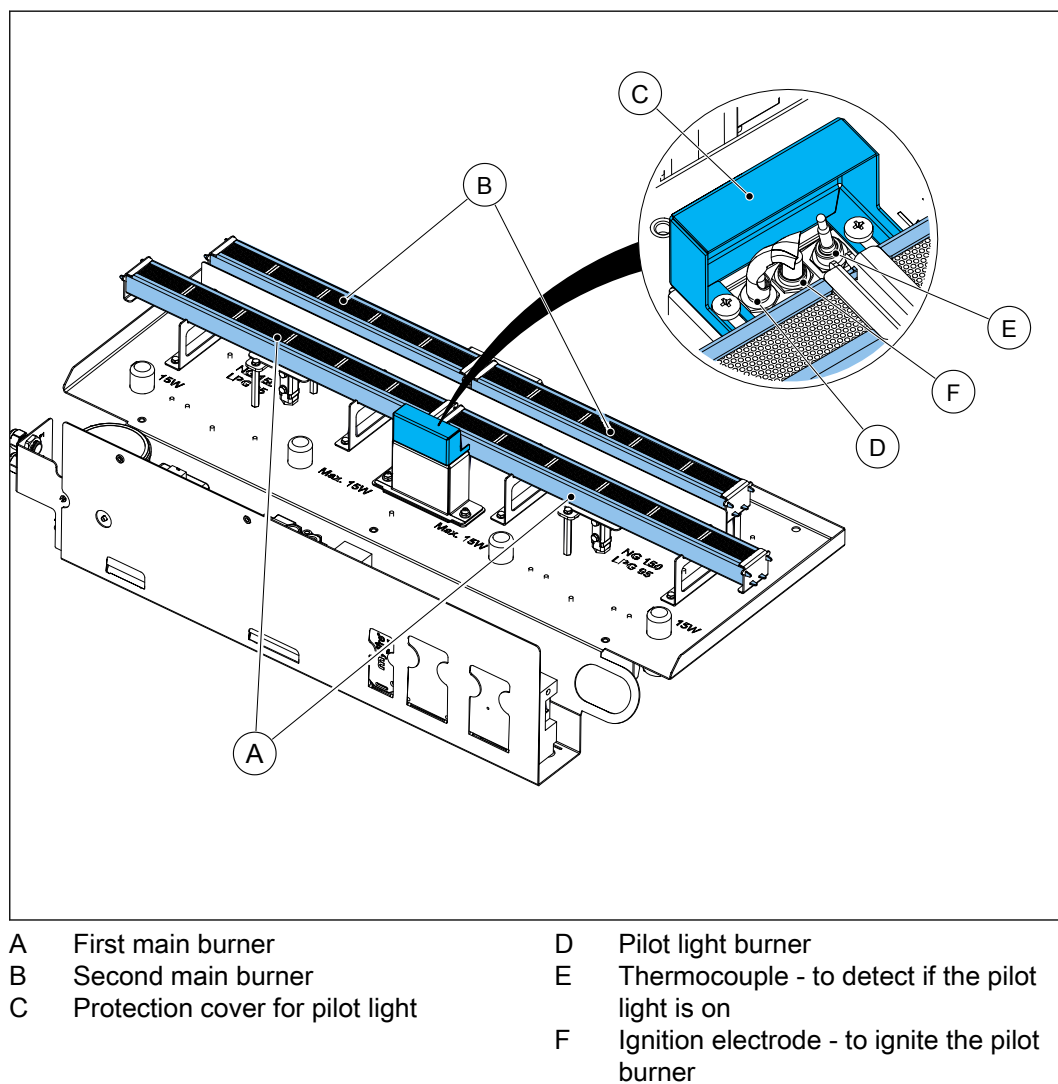
Figure 3. Burner bed and pilot light
