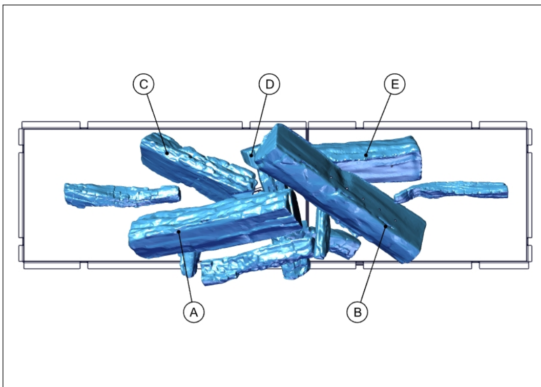
Figure 45. Position of ceramic wood logs and burners
