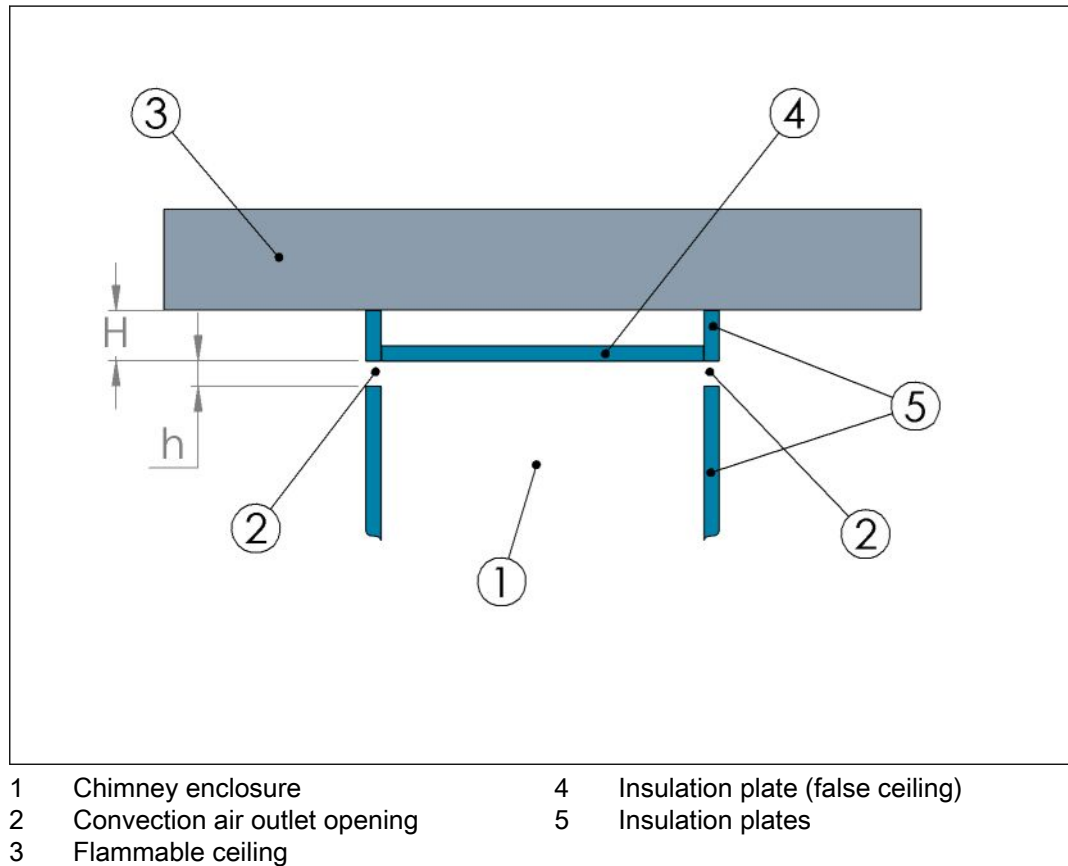
Figure 13. Clearances to flammable ceiling - Front view
