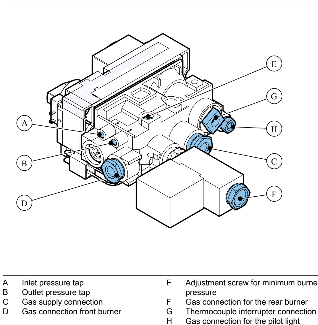
Figure 5. Gas regulator block (rear)
