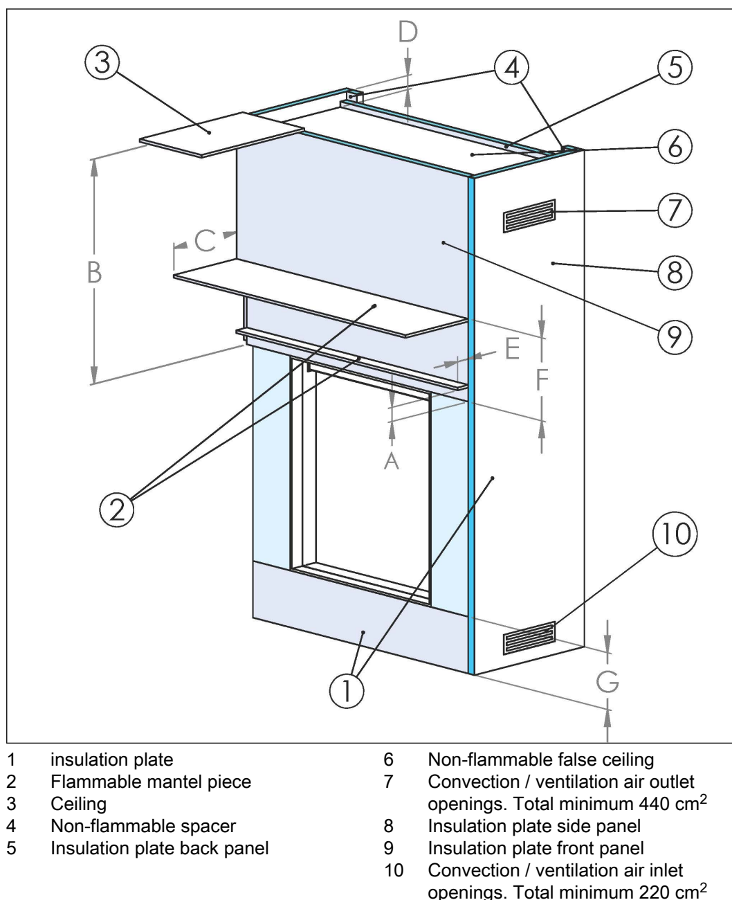
Figure 17. Mantel piece clearances
