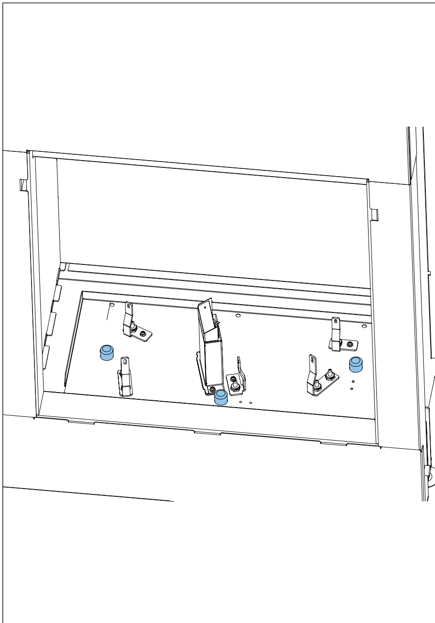
Figure 45. Position of ambient light bulbs
