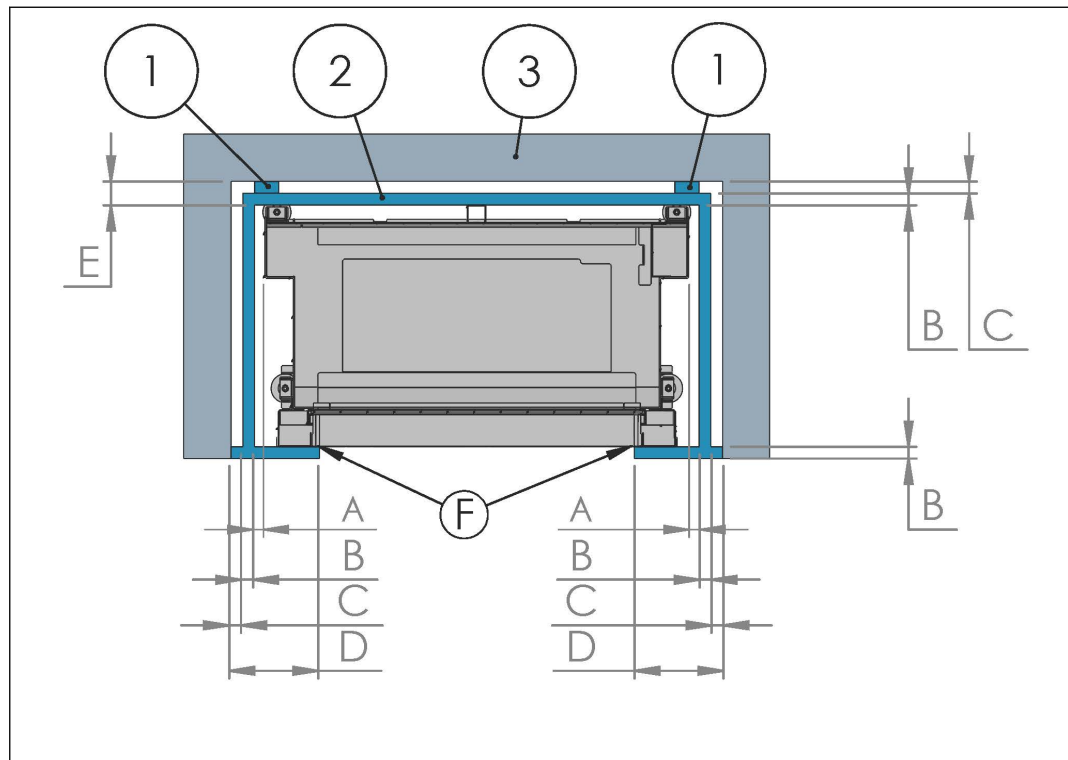
Figure 14. Clearances to non-flammable wall - Top view
