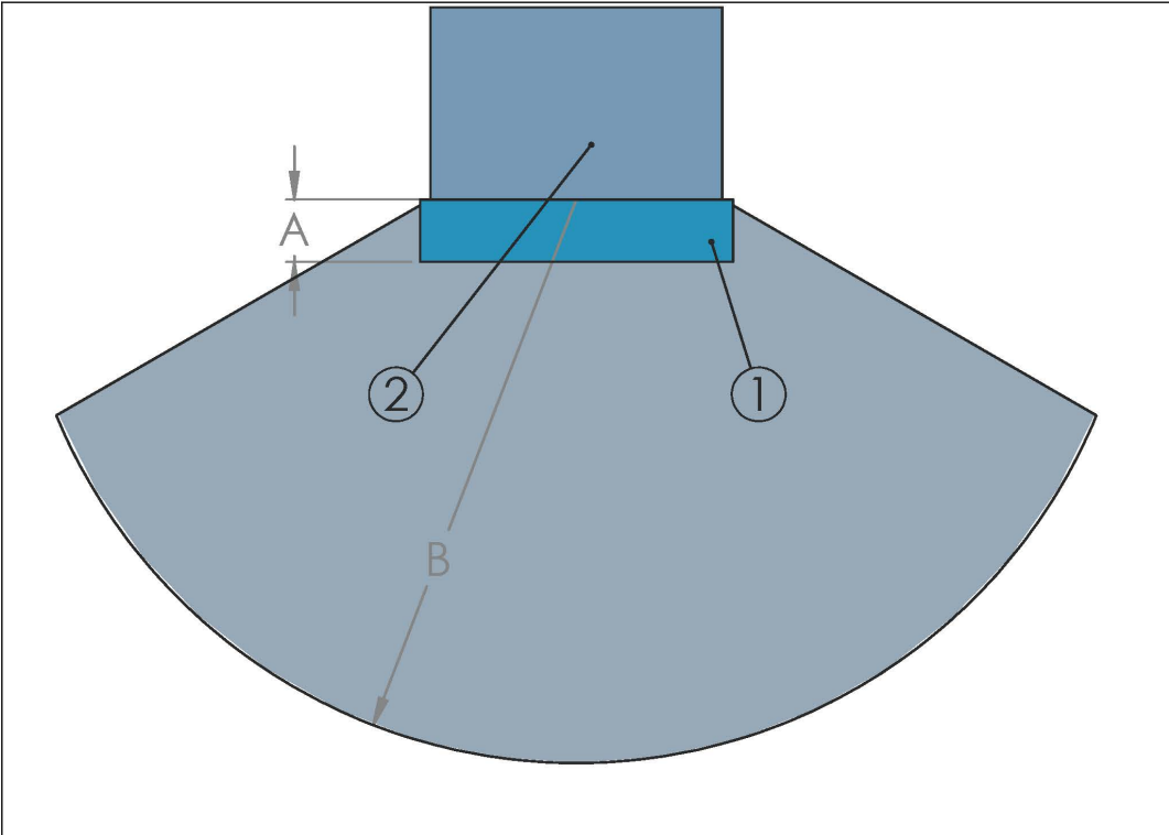
Figure 16. Minimum distances in front of the appliance
