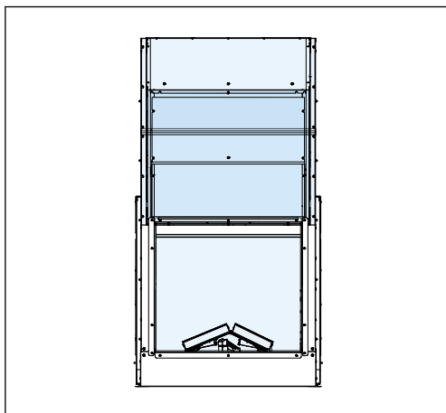
Figure 43. Fire screen in the service position
