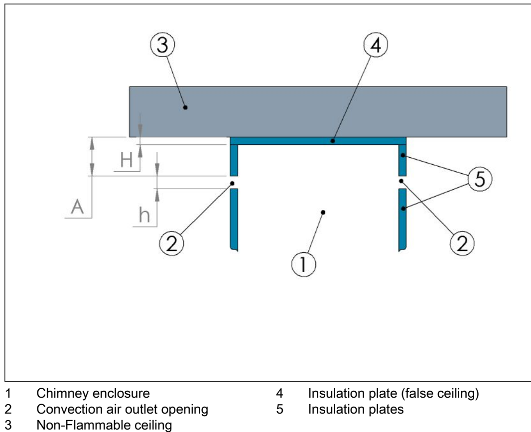
Figure 15. Clearances to non-flammable ceiling - Front view
