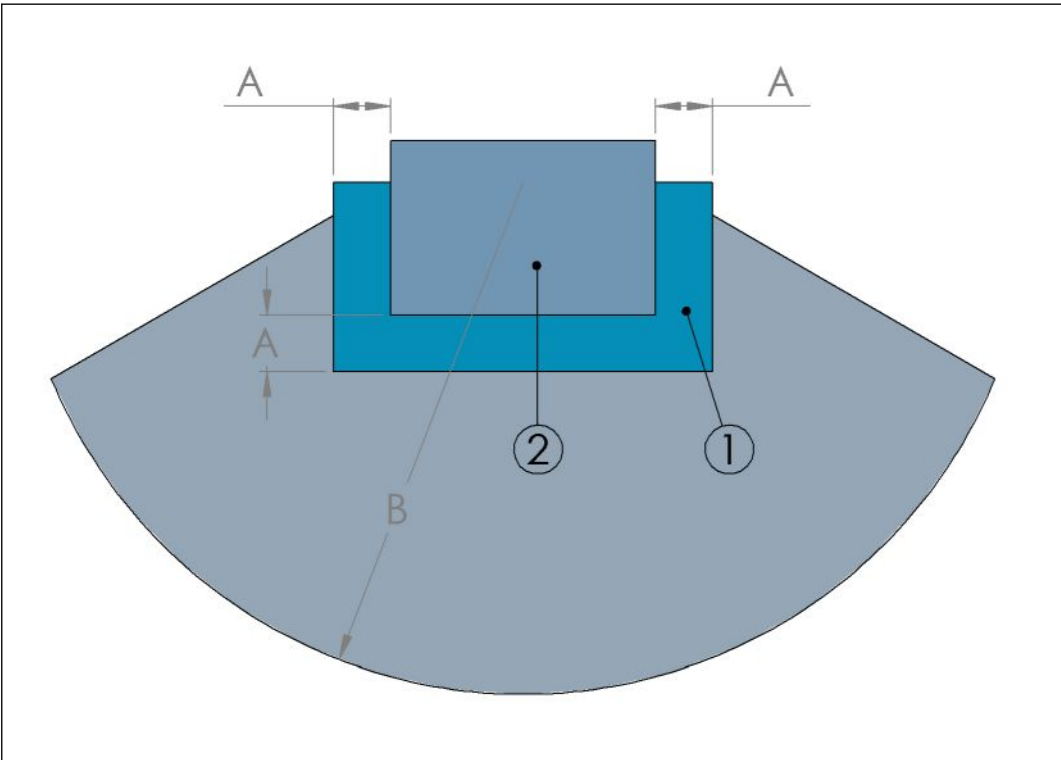
1 Non-flammable hearth (floor stone), minimum thickness 12 mm 2 Appliance
