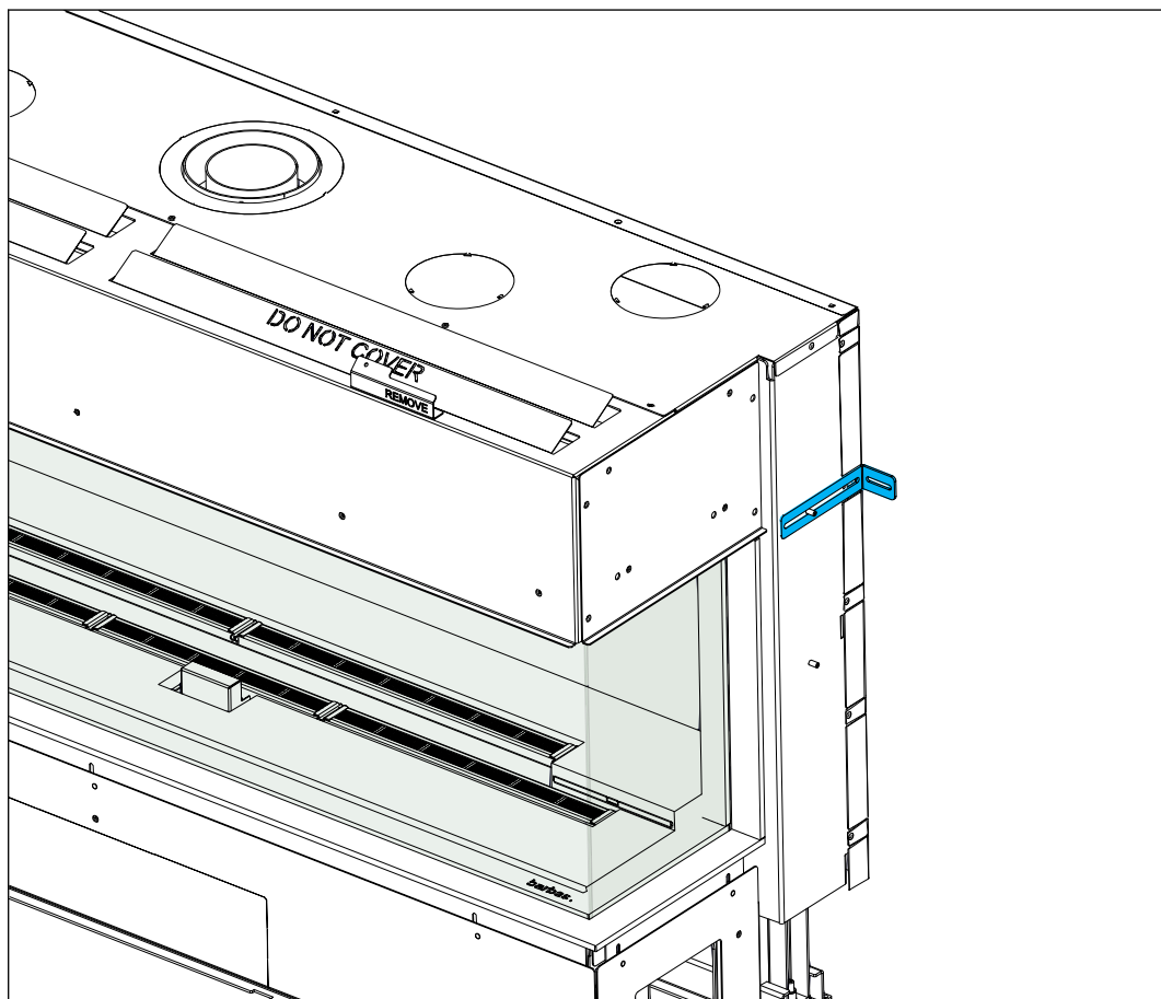
Figure 25. Attachment to the rear wall
