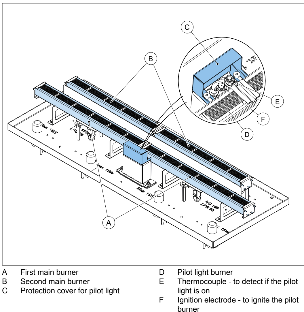
Figure 2. Burner bed and pilot light
