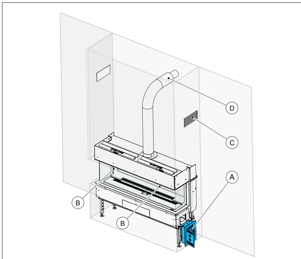
Figure 9. Typical installation of an appliance without convection set
