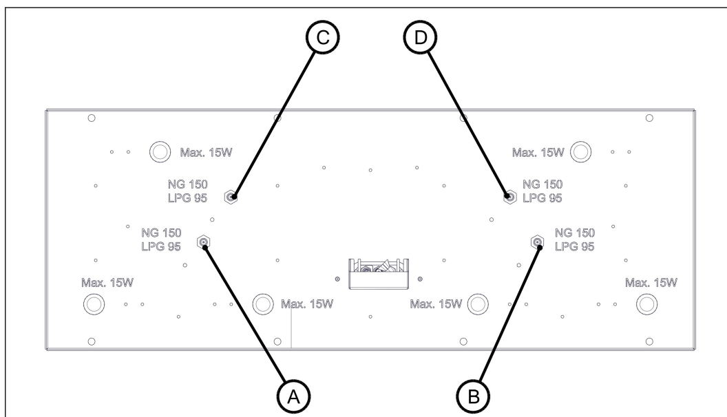
Figure 35. Position of primary air inlets and gas injectors
