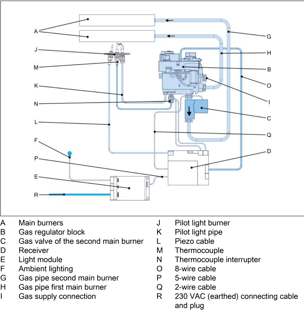
Figure 36. Diagram electrical and gas components
