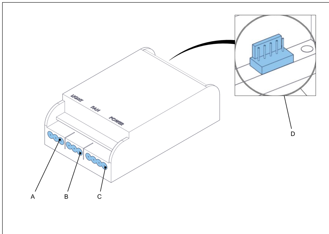
Figure 8. Fan/light module
