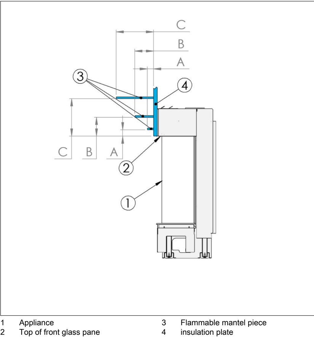
Figure 17. Top mantel piece clearances
