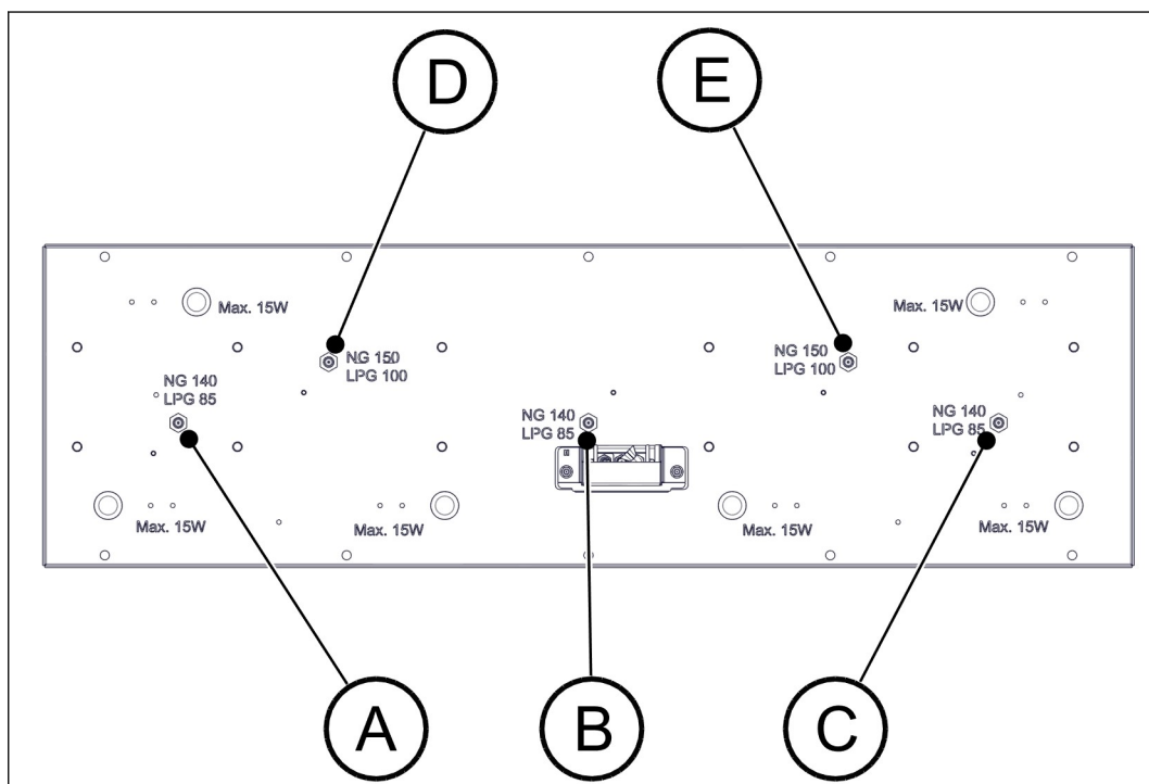
Figure 35. Position of primary air inlets and gas injectors
