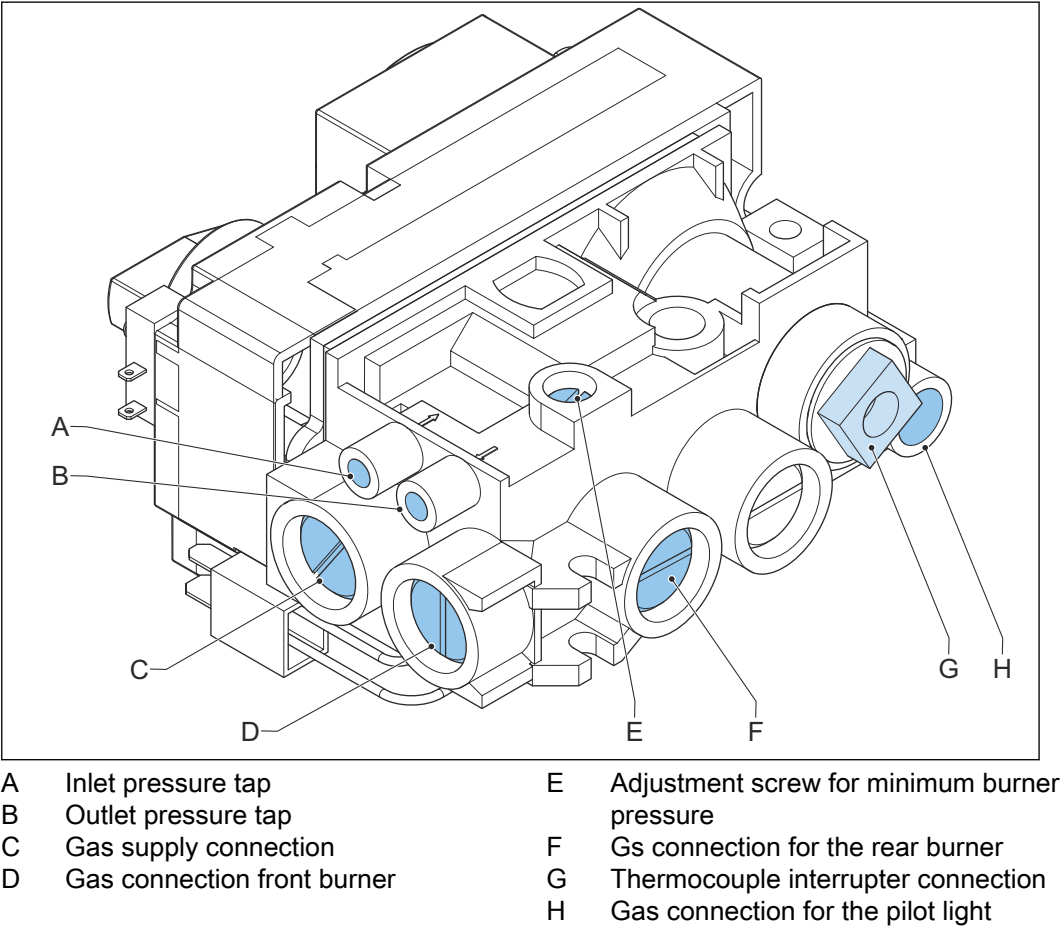
Figure 1. Gas regulator block (rear)
