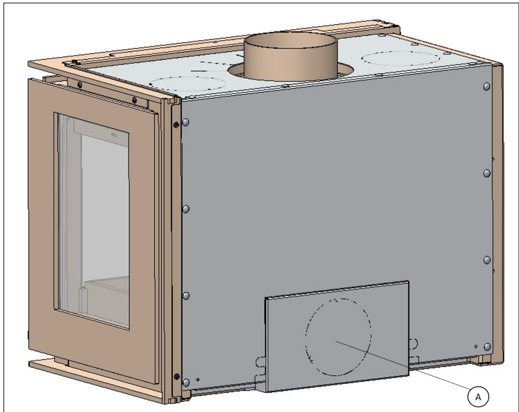
A Rear combustion air inlet
